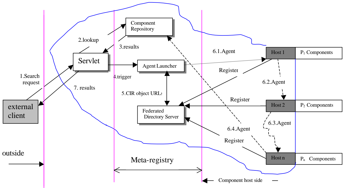
Figure 1: Architecture of Searching Component with Voyager Agent (CIR: Component-Info-Retrieval)
